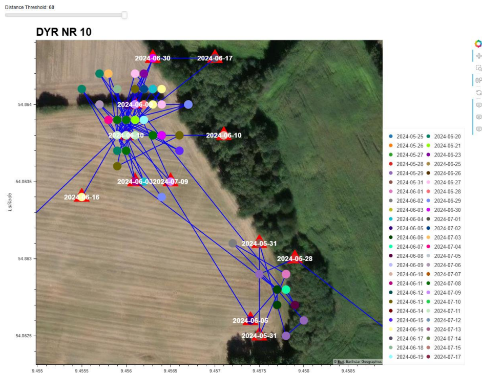
Figur 21.: No. 10: Day-centroid plot based on \text{sat} \geq 9 and Threshold 60 m. Significant movement shown by triangles
